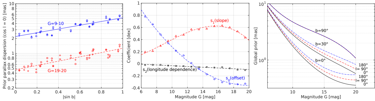
Fig. 4. Illustrations of the all-sky approximation to the parallax prior \sigma_{\pi, F90} as a function of galactic latitude b , for two magnitude ranges G = 9-10 (blue), and G = 19-20 (red). The small dependence on galactic longitude (the third term in Eq. (15)) has been subtracted leaving no systematic dependence on galactic longitude l , as shown by the different symbols ( \circ for \cos l > 0 , + for \cos l < 0 ). Middle: variations of the coefficients s_0 , s_1 , and s_2 with G magnitude, and polynomial fits according to Eqs. (16)–(18). Right: the prior \sigma_{\pi, F90} in Eq. (15) as a function of magnitude, for different latitudes (lowest to highest group: b = 0^\circ , 30^\circ , and 90^\circ ) and different longitudes (black solid l = 0^\circ , red dashed 90^\circ , blue dotted-dashed 180^\circ ).
