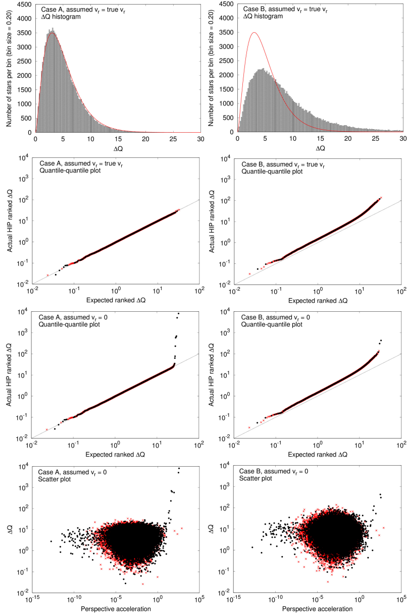
Fig. 4. Left column: Goodness of fit values \Delta Q for case A simulations. From top to bottom, the \Delta Q values (grey bars) follow a \chi^2 distribution (red line) with five degrees of freedom. If the assumed radial velocities in the solution equal the true values, the actual and expected distributions agree perfectly. If the assumed radial velocity is unknown (set to zero) deviations from the expected distributions are seen. These outliers are caused by perspective acceleration. The markers in the quantile-quantile and scatter plots correspond to stars with radial velocities from XHIP (black dots) and to stars with random radial velocities (red crosses). The three rightmost red crosses in the scatter plots correspond to HIP 80190, HIP 80194, and HIP 67694 which have very large uncertainties in the HIPPARCOS Catalogue. Therefore they do not show a large \Delta Q value even though they have large perspective acceleration. Right column: same plots for case B simulations (see Sect. 2.5).
